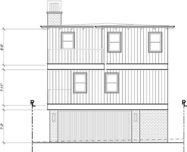
REAR EAST ELEVATION - CREST DRIVE 1/4" = 1'-0"
